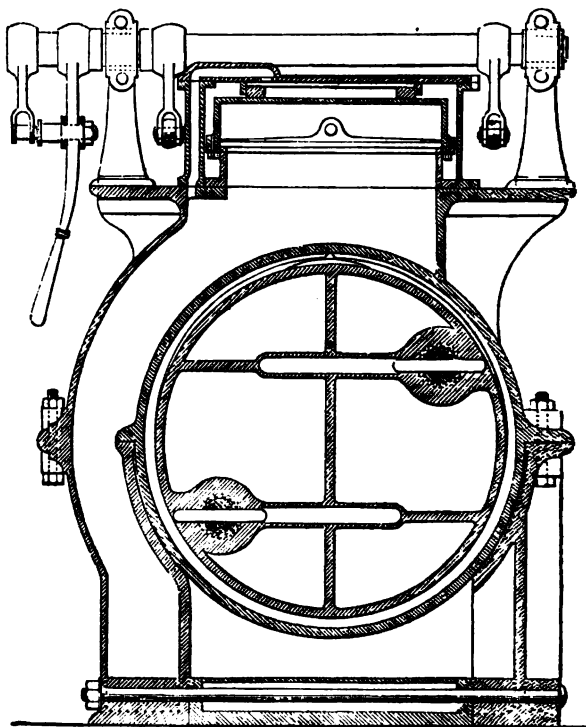
CROSS SECTION OF ONE OF THE CYLINDERS OF THE AMBRION.
