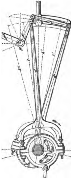
STEPHENSON'S LINK MOTION.
