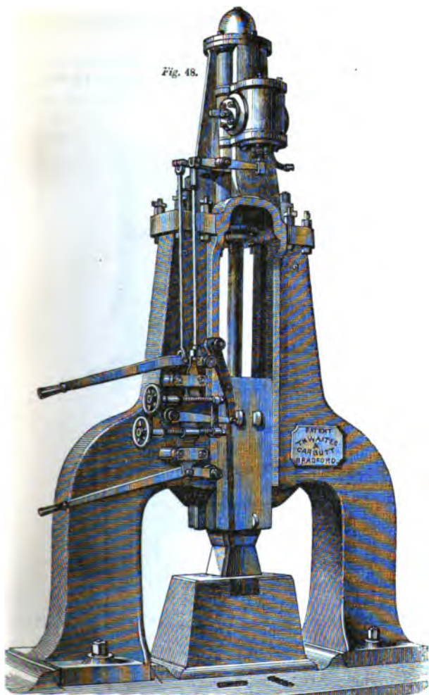
TWAINES AND CARBUTT'S HAMMER FOR HEAVY FORGINGS.
