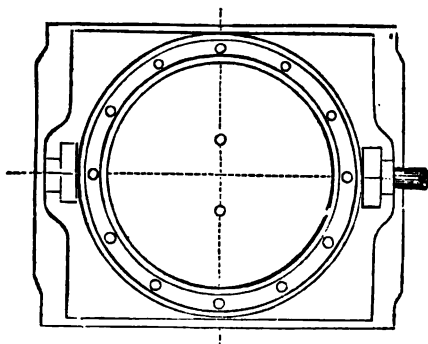
EQUILIBRIUM GRIDIRON SLIDE VALVE.
