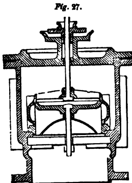
CORNISH EQUILIBRIUM VALVE.
