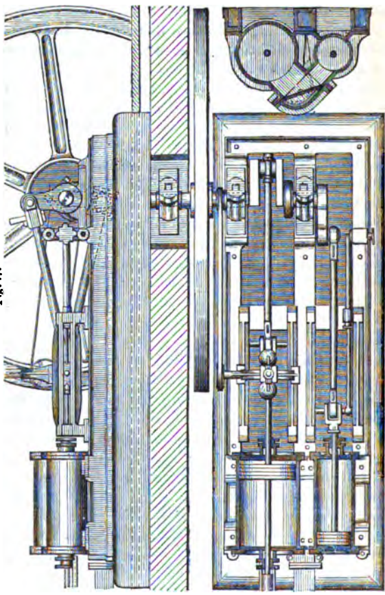
CARBETT, MARSHALL AND CO.'S BALANCED DOUBLE CYLINDER ENGINE. Elevation Ground Plan and Transverse Section.
