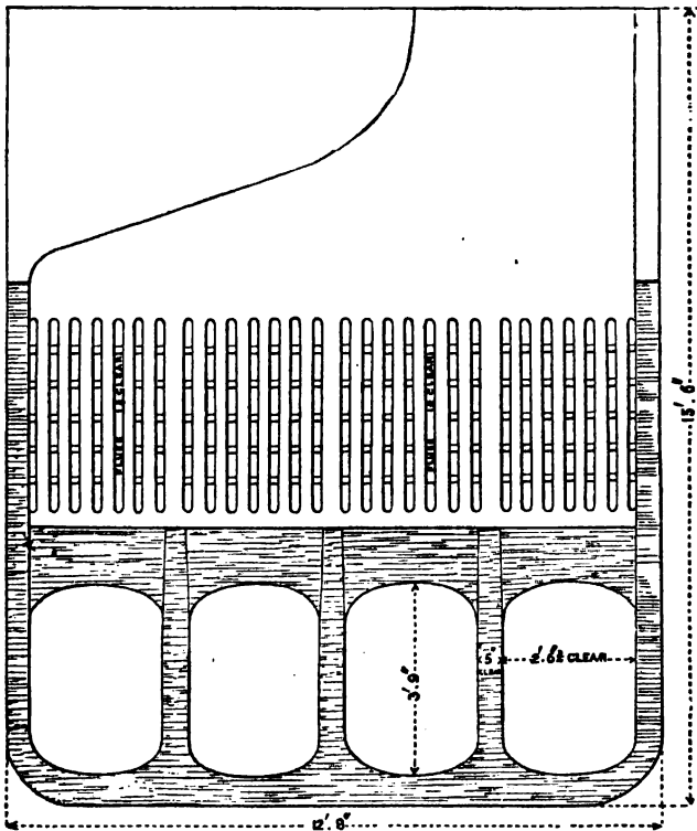
BOILERS OF STEAMER RIPON ON LAMB AND SUMMERS' PLAN. Transverse Section.
