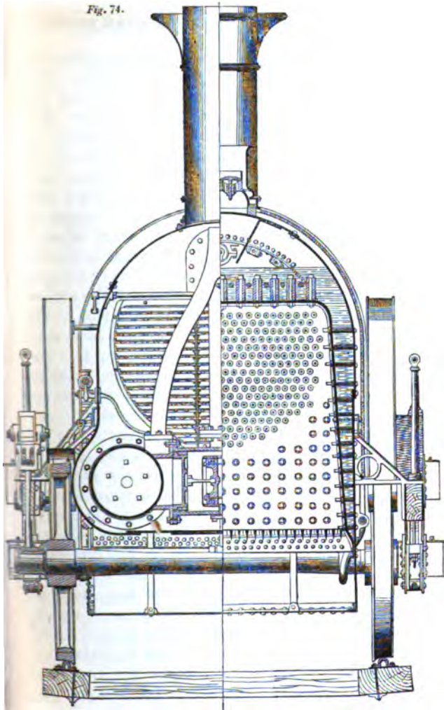
CROSS SECTION OF LOCOMOTIVE IRON DURE, GREAT WESTERN RAILWAY. M
