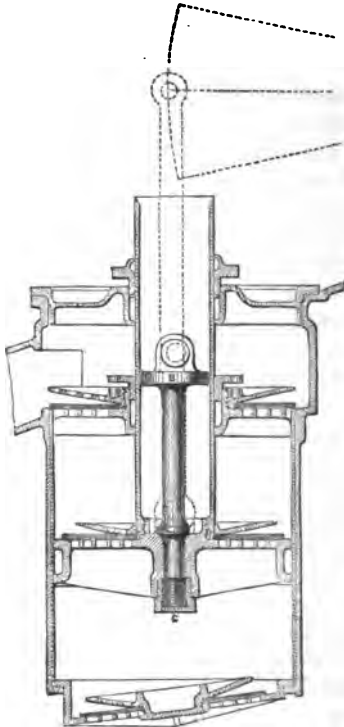
TRUNK AIR PUMP.
