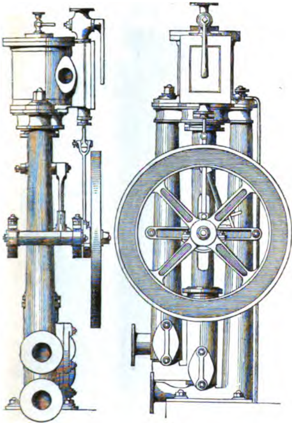
HAWTHORNE'S DONKEY ENGINE. Front and Side Views.
