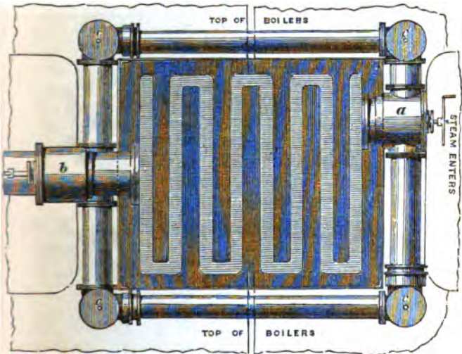
LAMB AND SUMMERS' SUPERHEATING APPARATUS, 1865. Ground Plan.
