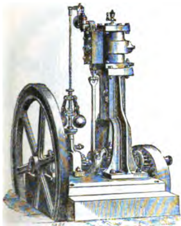
CARRETT, MARSHALL AND Co.'S FIXED PUMPING ENGINE FOR DEEP LIFTS.
