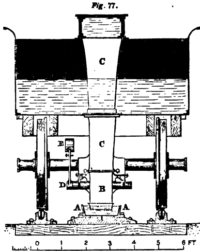
FEEDING SCOOP FOR RUNNING LOCOMOTIVES.
