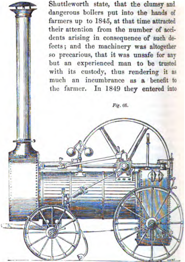
CLAYTON AND SHUTTLEWORTH'S PORTABLE ENGINE. Elevation.
