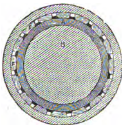
SCREW SHAFT BEARINGS; TRANSVERSE SECTION OF SHAFT AND PIPE AT STERN.
