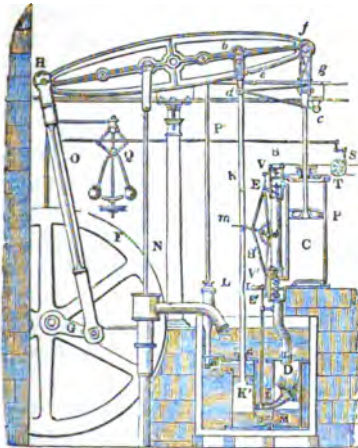
DOUBLE ACTING ROTATIVE STEAM ENGINE.
