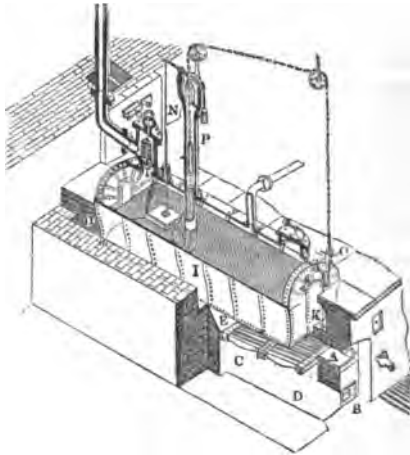
WAGGON BOILER.
