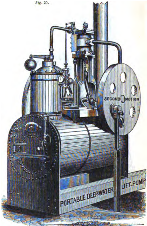
CARBETT, MARSHALL AND CO.'S PUMPING ENGINE AND BOILER.
