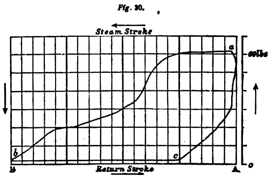
INDICATOR DIAGRAM.
