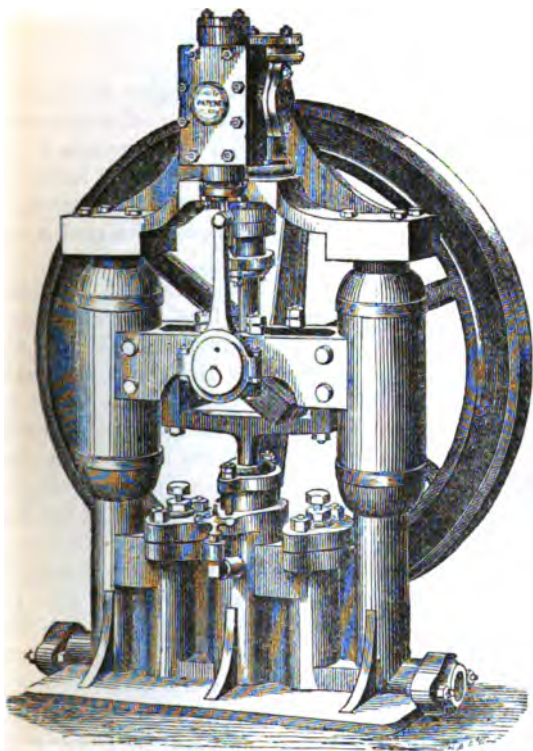
CASETT, MARSHALL AND CO.'S DONKEY FEED ENGINE.
